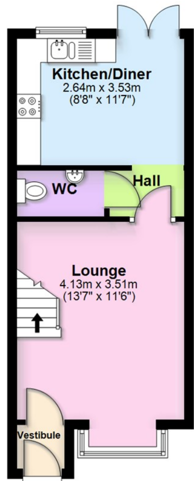
Ground Floor Approx. 29.4 sq. metres (316.6 sq. feet)
